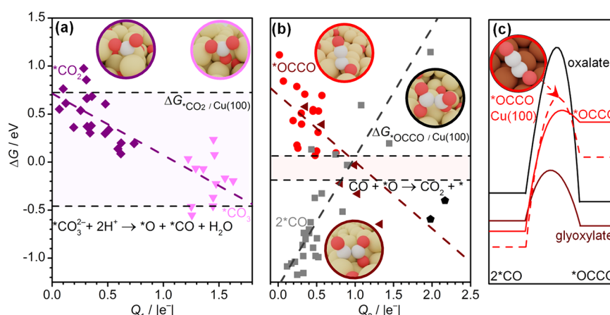
Figure 4. \text{CO}_2\text{R} activity and \text{C}_{2+} selectivity of OD-Cu versus ensemble polarization. (a) OD-Cu can adsorb \text{CO}_2 either on a Cu site (purple) or on a near-surface oxygen (magenta) forming a carbonate. \text{CO}_2 adsorption energy scales linearly with the polarization of the active sites, Q_1 : \Delta G_{\text{CO}_2} = +0.7(\pm 0.1) - 0.6(\pm 0.1)Q_1 . \text{Cu}^0\text{--Cu}^{\delta+} and \text{Cu}^{\delta+}\text{--Cu}^{\delta+} are responsible for enhancing OD-Cu \text{CO}_2\text{R} (purple area), while activity of \text{O}_{\text{ns}} sites is limited by carbonate formation. (b) Polarization of active ensembles, Q_2 , drives selectivity to \text{C}_2 products: \Delta G_{\text{OCCO}} = +0.7(\pm 0.1) - 0.7(\pm 0.1)Q_2 . A paired active site, \text{Cu}^{\delta+}\text{--O}_{\text{ns}} , stabilizes the \text{CO}\text{--CO} dimer as a glyoxylate-like intermediate (dark red), enhancing \text{C}_2 production. In contrast, for metallic Cu sites (red) \text{CO} dimerization is not favored, leading to a higher \text{CO} coverage (gray), \Delta G_{2\text{CO}} = -1.3(\pm 0.1) + 1.3(\pm 0.1)Q_2 . For very strong polarization, stable oxalates are generated on the surface (black). Q_1 and Q_2 are defined as the sum of absolute Bader charges of the atoms in the ensemble calculated with implicit solvation (eqs S21 and S22, Figure S27). (c) \text{OCCO} intermediate on both OD-Cu and Cu(100) and oxalate formation on OD-Cu presents a high kinetic barrier of more than 1 eV. The pathway toward the glyoxylate-like intermediate has instead a mild barrier of 0.53 eV. Potential and dipole corrections, here not included, stabilize all intermediates similarly (Table S16). Further details on the linear regressions are shown in Table S17.
