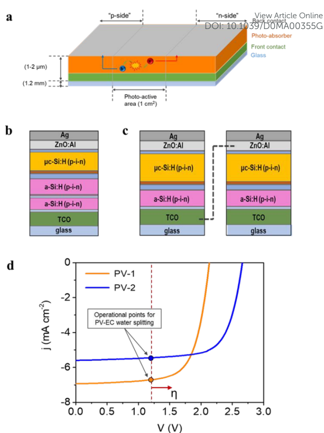
Figure 4. a. Schematic representation of the photovoltaic device design, where the Ag contacts are outside of the 'photo-active area', and serve to transport the photogenerated charge carriers to the electrocatalyst. The photo-active region, with a size of 1cm 2 , consists of a Si-based device. The architecture of the two different devices employed: b. The a-Si:H/a-Si:H/ \mu c-Si:H triple-junction solar cell (PV-1) and c. The module of two a-Si:H/ \mu c-Si:H tandem cells connected in series (PV-2). d. Characteristic current-voltage curves of PV-1 and PV-2 devices. The theoretical operational points of the integrated PV-EC water splitting devices are represented (the dashed line indicates the water splitting thermodynamic potential at 1.23 V). The red arrow indicates that the "practical" operating point is shifted due to overpotentials ( \eta ).
