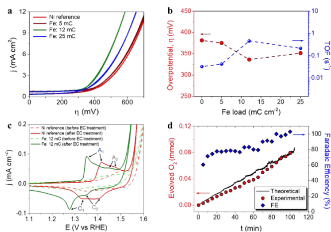
Figure 1. a. Cyclic voltammetry measurements, recorded with a scan rate of 10 mV s -1 , for the different samples prepared with different electrodeposited Fe charges. b. Overpotential ( \eta ) for the water oxidation onset and turn-over frequency (TOF), calculated at an overpotential of 400 mV, as a function of the Fe content on the Ni-based electrocatalysts. c. Effect of electrochemical activation on reference Ni foil thermally treated and optimal Ni-Fe electrocatalyst before (dashed lines) and after (solid lines) electrochemical activation (50 cycles). d. Oxygen evolution measurement and faradaic efficiency (FE), performed with the optimal Ni-Fe catalyst (Fe load: 12 mC cm -2 corresponding to 1.06 at-% Fe content), after activation at 1.6 V vs RHE.
