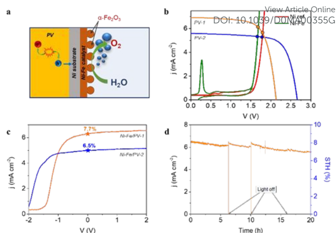
Figure 5. a. Schematic representation of the general operation of the integrated PV-EC photoanode, obtained by the direct coupling of the Si-based solar device and the Ni-Fe optimized catalyst. b. Estimation of the theoretical operation point from the characteristic current-voltage curve of the photovoltaic devices and LSV of the reference Ni sample and the optimal electrocatalyst (Ni-Fe), measured in a two-electrode configuration. c. LSV recorded in two-electrode configuration at 50\text{ mV s}^{-1} , of the integrated PV-EC devices as photoanodes and STH efficiencies. d. Stability test of the integrated photoanode combining the optimal Ni-Fe electrocatalyst and the PV-1 showing promising stability for more than 20 hours under continuous operation. The left y-axis shows the recorded photocurrent density, while the right y-axis represents the calculated STH efficiency.
